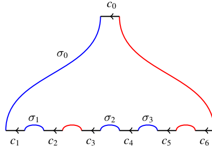
Figure 1: Differential in CE^* , The word \sigma_0 c_1 \sigma_1 c_2 c_3 \sigma_2 c_4 \sigma_3 c_5 c_6 appears in dc_0 .
