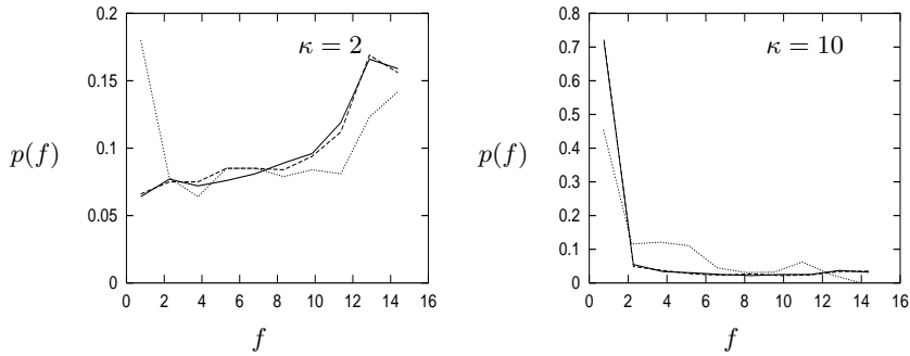
Fig. 2. The distribution p(f) of antibody concentrations, for the finitely connected network with \kappa = 2 (left) and \kappa = 10 (right). We compare the solutions of the Liouville equation (two examples, solid and dashed) with the results of numerical simulations (at N = 800 , dotted).
