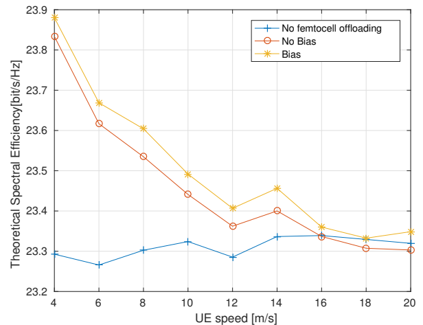
Fig. 7: Theoretical Spectral Efficiency as a function of the vehicular traffic speed v .
