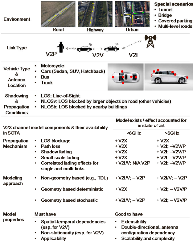
Fig. 2: V2X-specific considerations for channel modeling. For each link type (V2V, V2P, V2I), we indicate whether an appropriate model exists (“+”) or not (“-”) in the literature. For further details, see [2], [3], [4].
