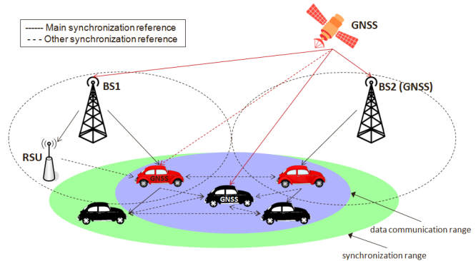
Fig. 3: Scenario with in- and out-of-coverage vehicular users. GNSS may be available to some base stations, RSUs and users. Synchronization source selection and distributed synchronization are used to achieve global synchronization.
