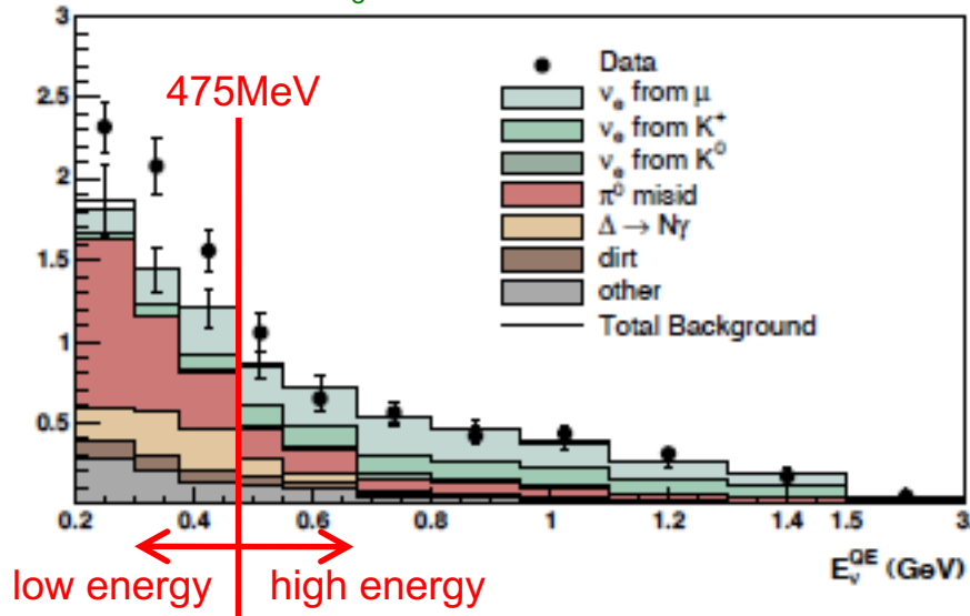
MiniBooNE low E \nu_e excess
