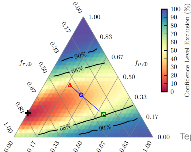
IceCube flavour triangle diagram
