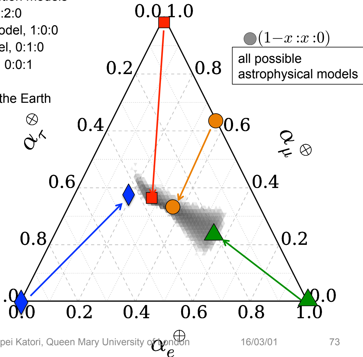
IceCube flavour triangle diagram
