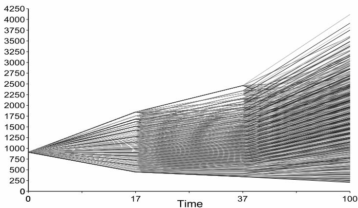
Figure 1: Scenario tree with branching structure (50, 10, 10).
