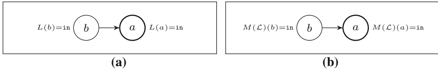
Fig. 10 Counter-example used in proposition 5(v). a Agent's labelling \mathcal{L} . b Labelling profile M(\mathcal{L})
