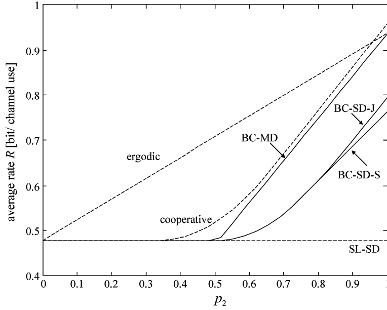
Fig. 2. Average achievable rates (2) for the proposed BC-based schemes with single description (SD) and either separate (S) or joint (J) decompression/ decoding, or multidescription (MD) compression, versus the probability p_2 = 1 - p_1 of having M = 2 active links. For reference, the upper bound (12) achievable with cooperative relay, the upper bound (27) corresponding to ergodic link failures and the rate (28) of single-layer (SL), or nonbroadcast, transmission with SD compression are also shown ( P = 15 dB and C = 0.5 ).
