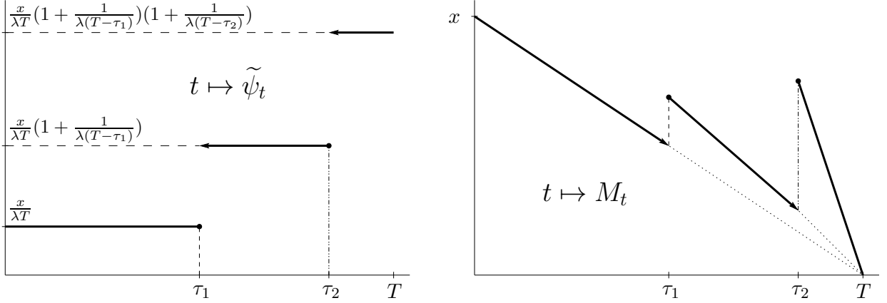
FIGURE 1. A schematic representation of typical paths of the integrand \tilde{\psi} and the local martingale M = x + \int_0^T \tilde{\psi}_u dX_u .
