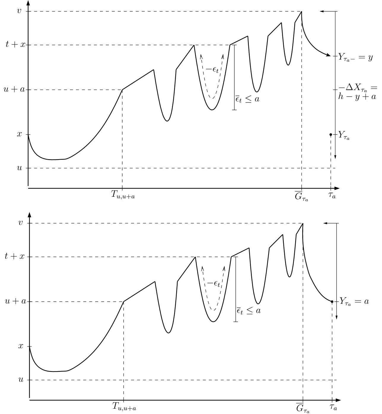
FIGURE 1. The top figure contains a schematic representation of a typical path of the process X in the event A_o = \{\underline{X}_{\tau_a} \geq u, \bar{X}_{\tau_a} \in dv, Y_{\tau_a-} \in dy, Y_{\tau_a} - a \in dh\} . This figure illustrates the idea behind the proof of Theorem 1: the depicted path satisfies T_{u,u+a} = T_{u+a}^+ and T_v^+ = \bar{G}_{\tau_a} . It is clear from the figure that the trajectory can be decomposed into the following three parts, each of which is analysed separately in the proof of Theorem 1: (1) the segment over the interval [0, T_{u,u+a}] , (2) the jump at time \tau_a and (3) the segment that straddles \bar{G}_{\tau_a} over the time interval (T_{u,u+a}, \tau_a) . The bottom figure depicts a schematic representation of a typical path of the process X in the event A_c = \{\underline{X}_{\tau_a} \geq u, \bar{X}_{\tau_a} \in dv, Y_{\tau_a} = a\} .
