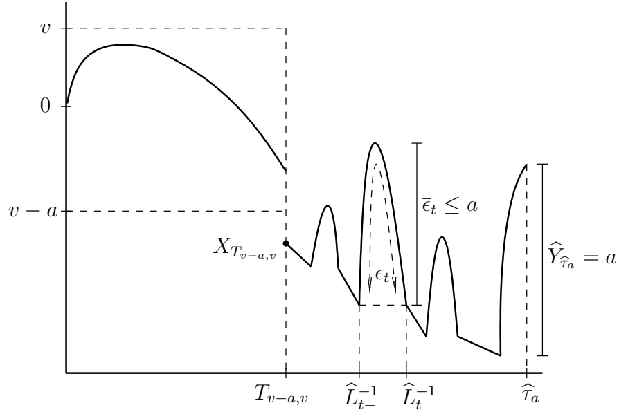
FIGURE 2. A schematic representation of a path which satisfies T_{v-a,v} = T_{v-a}^- and is therefore in the event \{\bar{X}_{\hat{\tau}_a} < v\} . At the moment of local time t the path in the figure has an excursion \epsilon_t away from the infimum. The process \hat{L}^{-1} is the inverse local time at zero for the Markov process \hat{Y} .
