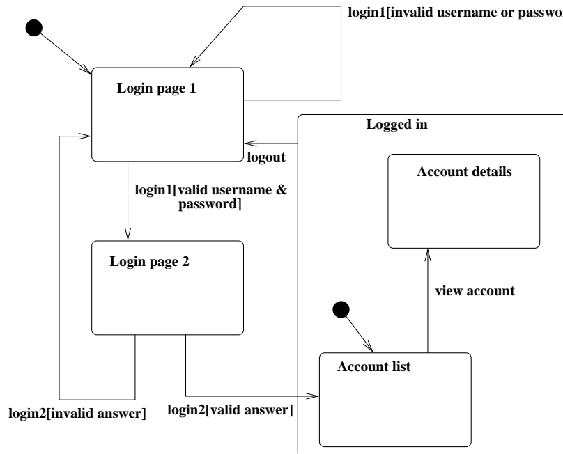
Figure 1: Bank website state machine
