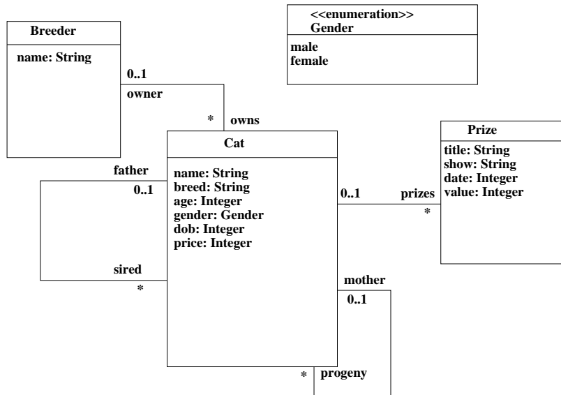
Figure 1: Cattery class diagram
