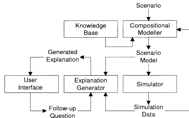
Figure 9 Architecture of a self-explanatory simulator
