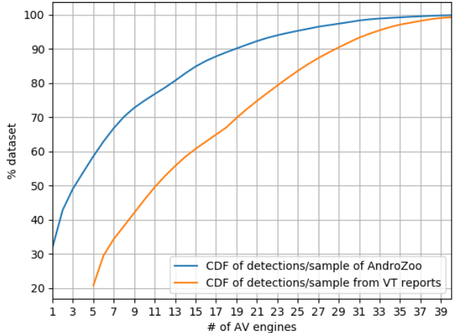
Fig. 1: CDF of AV detections for samples in our dataset. x-axis represents # of engines detecting samples, y-axis is the percentage of samples in dataset detected by this # of engines.
